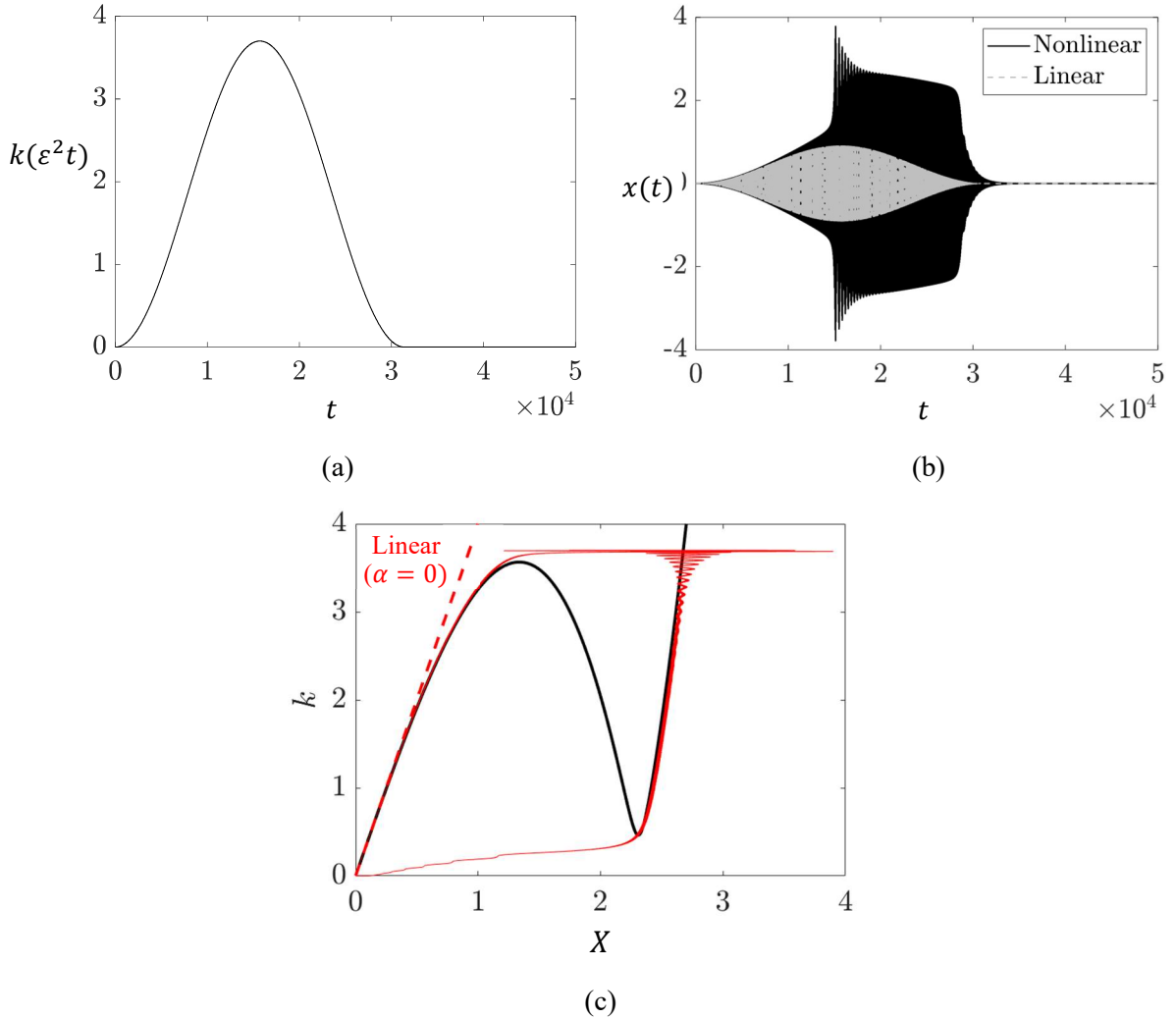
Figure 2. Response of oscillator (9) for zero initial conditions subject to the super-slow cycle of modulated forcing magnitude depicted in (a): Strongly modulated nonlinear and linear responses (b), and projection of the modulated response amplitude onto the SIM (c); the super-slow tracking of the hysteresis loop in this case is evident.
