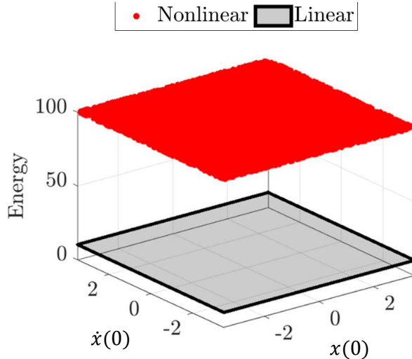
Figure 7. Insensitivity of the response depicted in Fig. 2 (with corresponding energy intake shown in Fig. 3b) to the initial conditions.
