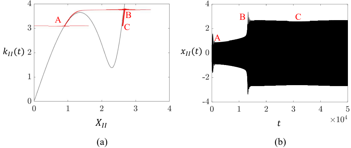
Figure 5. Response of (9) due to the modulated forcing magnitude k_{II}(\varepsilon^2 t) : (a) Projection of the forced dynamics on the SIM, and (b) corresponding super-slow modulated response x_{II}(\varepsilon^2 t) ; note the drastically increased response compared to Fig. 4b, caused by a slight increase in the modulation of the forcing magnitude.
