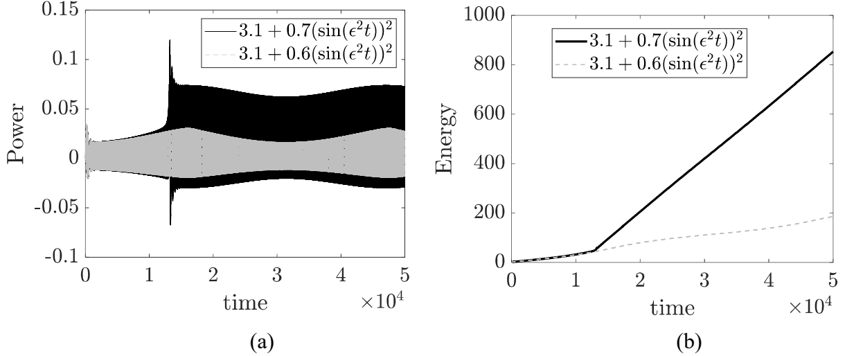
Figure 6. Power input (a) and energy intake (b) in the oscillator (9) for applied harmonic forcing with magnitude modulations k_I(\varepsilon^2 t) and k_{II}(\varepsilon^2 t) ; these results correspond to the responses presented in Figs. 4 and 5.
