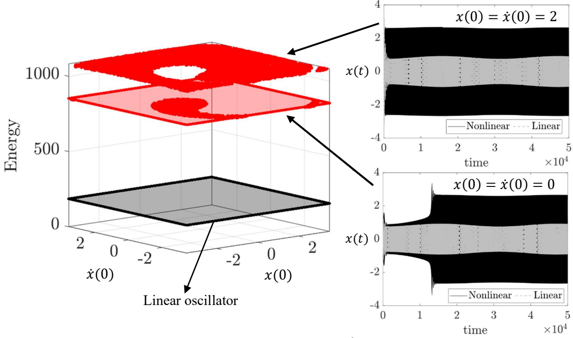
Figure 8. Dependence of the response depicted in Fig. 4 (with corresponding energy intake shown in Fig. 6) to the initial conditions; a representative realization for each of the two types of responses is shown on the right.
