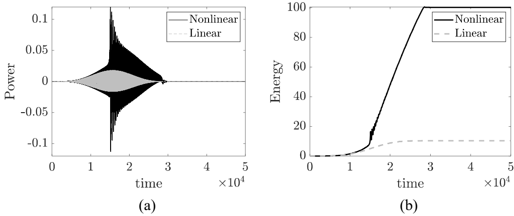
Figure 3. Power (a) and energy intake (b) (normalized units) in the oscillator (9) with zero initial conditions, and subject to the super-slow cycle of modulated force depicted in Fig. 2a; the corresponding results for the linear system ( \alpha = 0 ) are shown for comparison.
