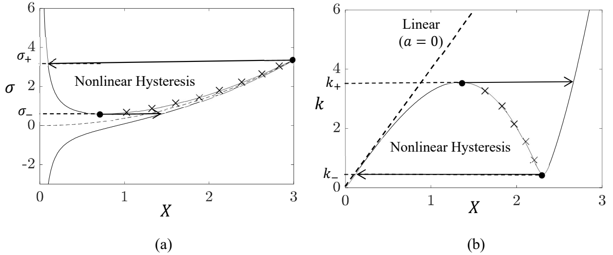
Figure 1. Approximate steady state of the forced oscillator (1) (slow invariant manifold – SIM) for \zeta = 0.1 and a = 1 : (a) Response amplitude versus frequency detuning for fixed forcing amplitude k = 0.6 , and (b) response amplitude versus forcing magnitude for fixed frequency detuning \sigma = 2.0 (for comparison, the corresponding linear invariant manifold is depicted by dashed line); nonlinear hysteresis loops are being formed in the bi-stability regions of the two plots, bounded by the fold points which are denoted by bullets ( \bullet ), while the unstable branches are denoted by crosses ( \times ).
